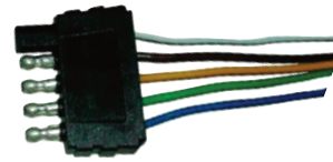
5 Pole Flat Connectors 27020
